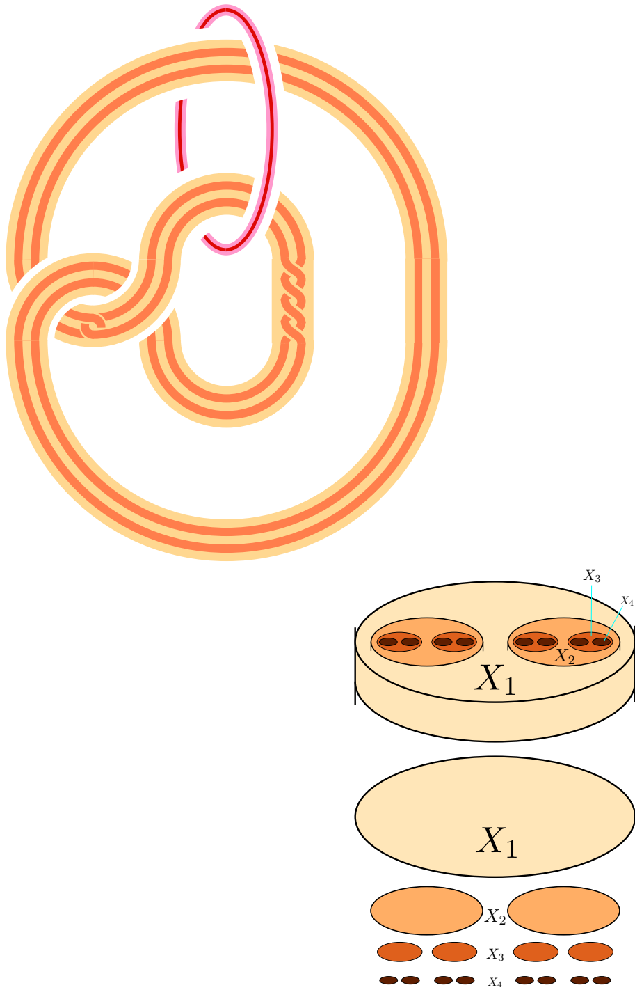
Figure 3: Whitehead link W_n , X_n
