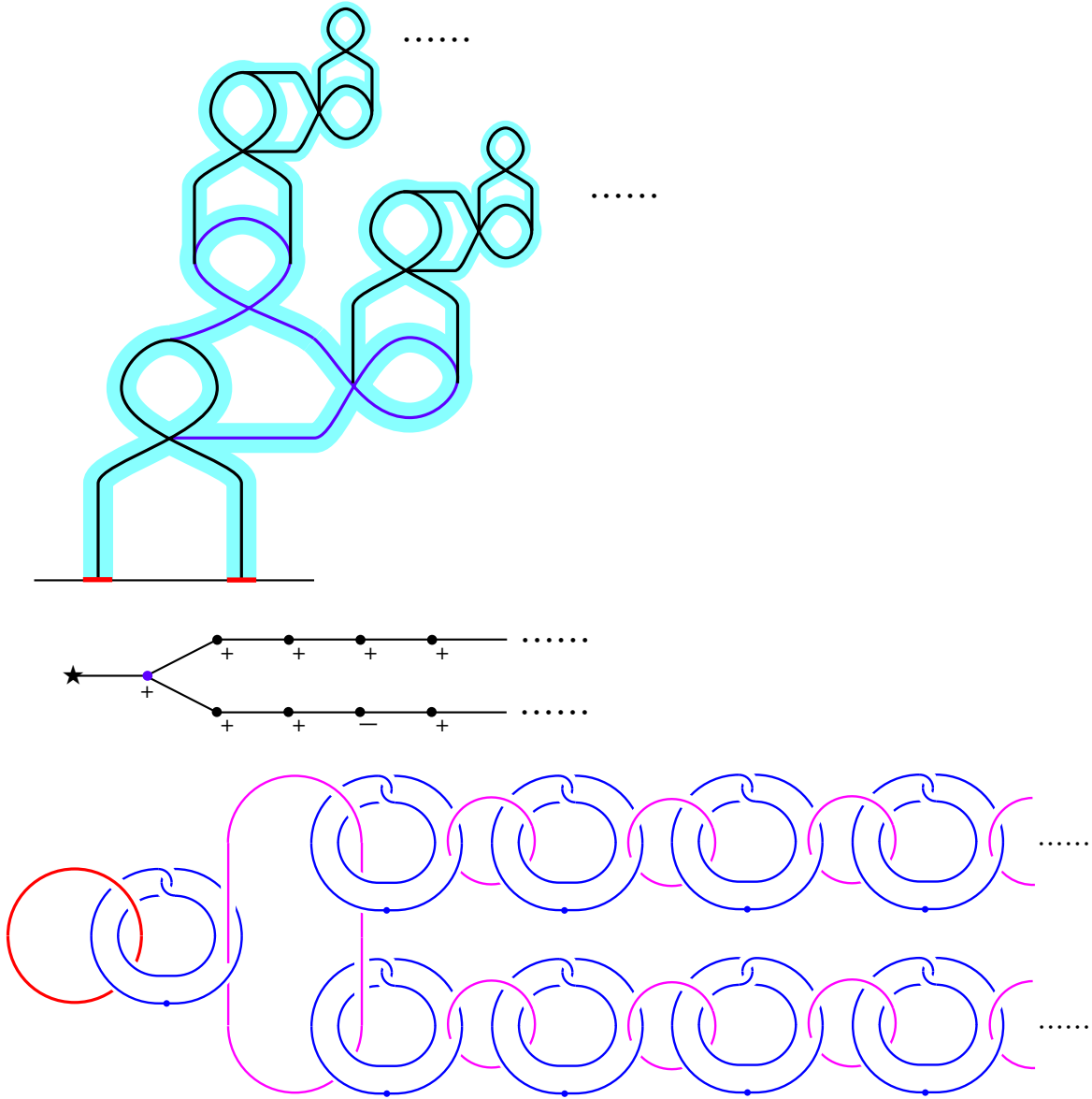
Figure 9: Another Type CH その2
