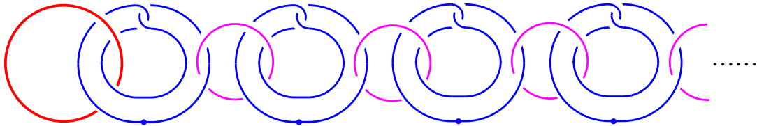
Figure 1: Diagram of the simplest CH
