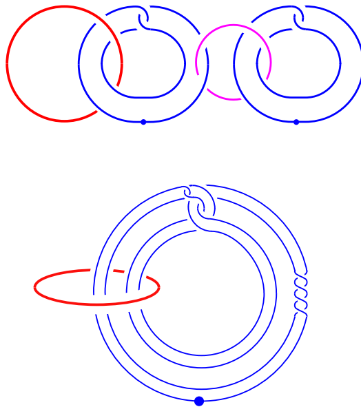
Figure 2: 2nd Whitney tower \leftrightarrow Whitehead link Wh_2
