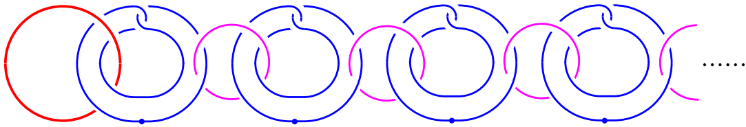
Figure 1: Diagram of the simplest CH
