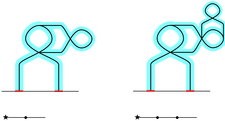
Figure 5: The 2nd/3rd Whitney Tower
