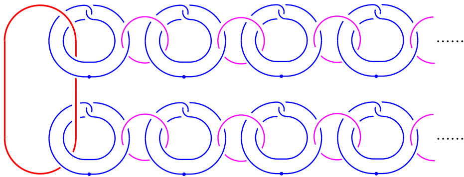
Figure 7: Another Type CH その 1
