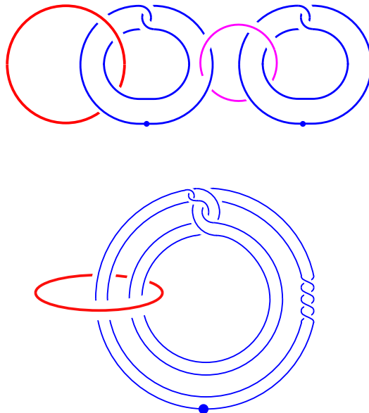
Figure 2: 2nd Whitney tower \leftrightarrow Whitehead link W_2
