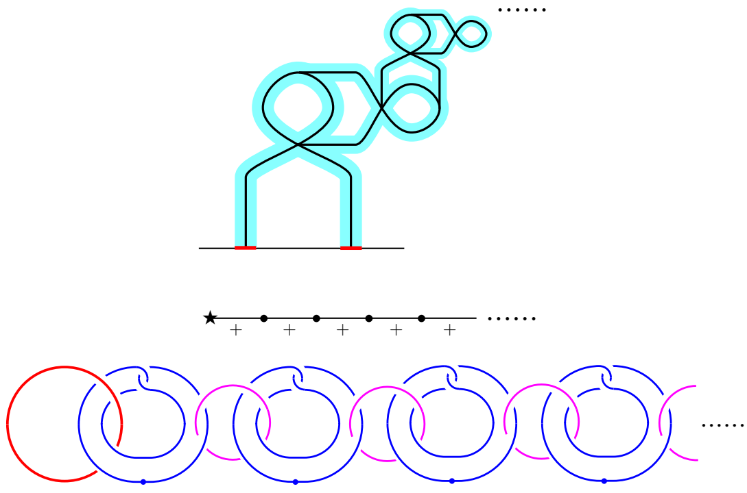
Figure 6: The simplest CH (with signs)
