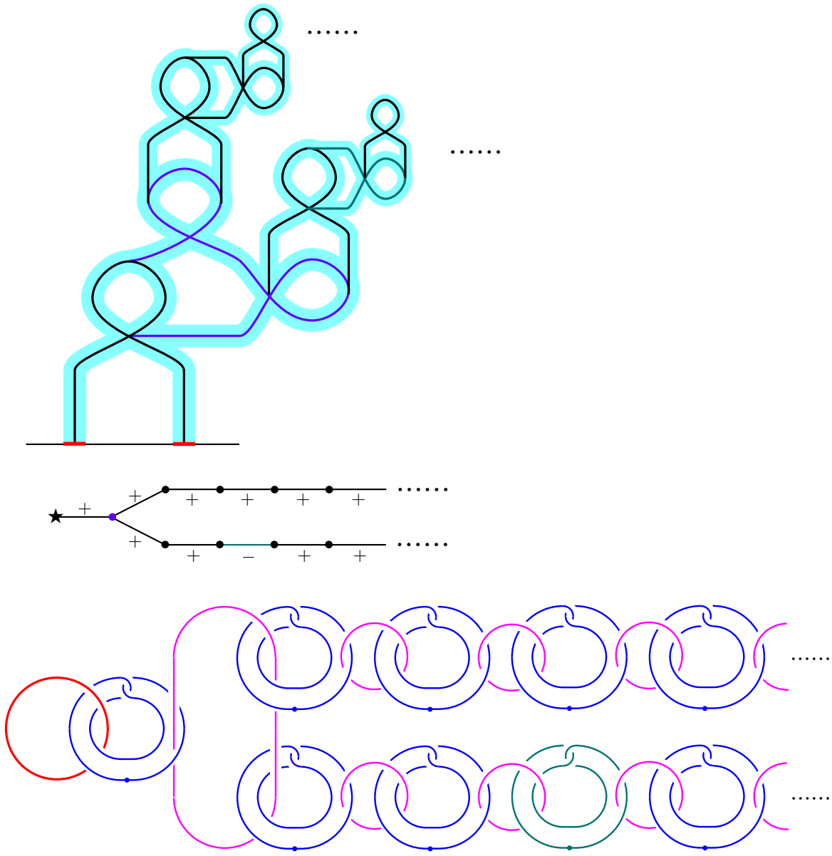
Figure 9: Another Type CH その2
